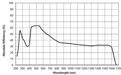
1200 Line VIS Holographic
